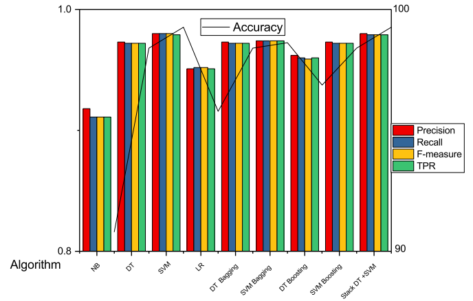
Fig. 3: Test Results various ML algorithms
